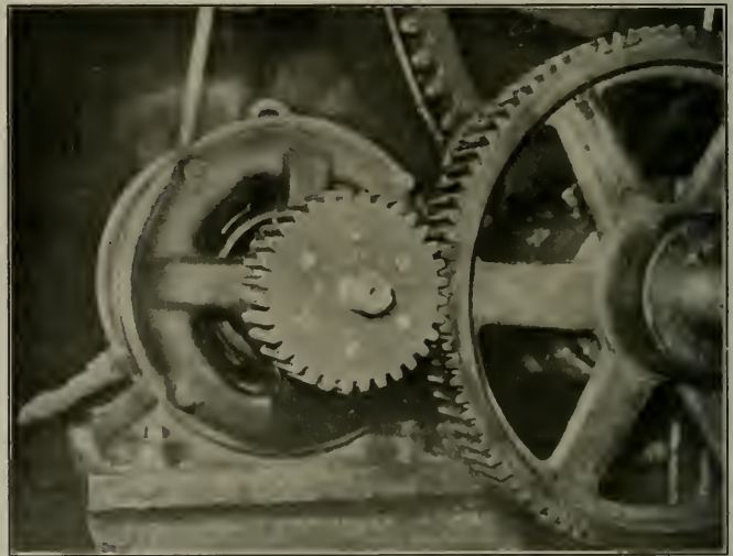
FIG. 4. PINION FOR DRIVING PUNCH PRESS: 4 DP. 32 TEETH ON 7\frac{1}{2} HORSE POWER MOTORS
